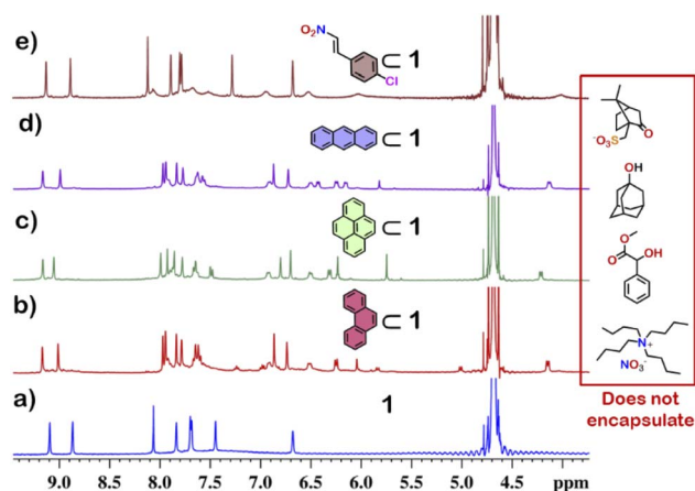
Fig. 4 Partial 1 H NMR stack plot of (a) 1 , (b) P ⊂ 1 ( P : phenanthrene), (c) pyrene⊂ 1 , (d) A ⊂ 1 ( A : anthracene) and (e) Ns ⊂ 1 ( Ns : (E)-1-chloro-4-(2-nitrovinyl)benzene) in D 2 O showing the change in NMR by guest encapsulation. (Inset) examples of non-planar guests that could not be encapsulated by 1 .
