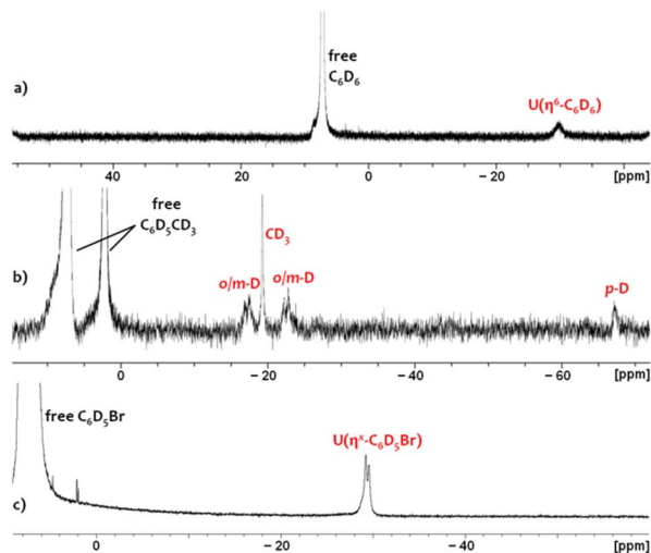
Fig. 5 ^2\text{H} NMR spectra of (a) 2-d 6 in \text{C}_6\text{H}_5\text{Br} containing 5 equiv. of \text{C}_6\text{D}_6 , (b) 3-d 8 in \text{C}_6\text{H}_5\text{Br} containing 5 equiv. of toluene- d_8 , and (c) 4-d 5 in neat \text{C}_6\text{D}_5\text{Br} .
