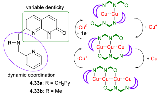
Scheme 41 Dynamic polynucleating ligands based on naphthyridone backbone and schematic representation of the stepwise growth of multicopper(i) chains by “sliding” naphthyridonate fragments along the growing chain.
