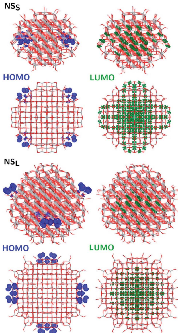
Fig. 11 Side (upper) and top (lower) views of the electronic density plots of the frontier orbitals of \text{NS}_5 and \text{NSL} (isosurface = 5 \times 10^{-4} au, except for HOMO, for which isosurface = 1 \times 10^{-3} au). Reprinted with permission from G. Fazio, L. Ferrighi and C. Di Valentin, J. Phys. Chem. C , 2015, 119 , 20735–20746. Copyright 2015 American Chemical Society.
