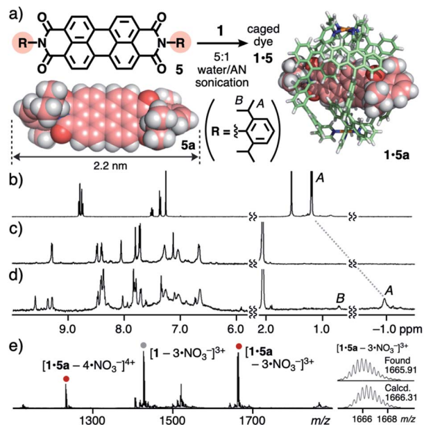
Fig. 4 (a) Formation of caged dye 1·5 and the optimized structures of 5a and 1·5a ( R^1 = H for clarity). ^1H NMR spectra (500 MHz, 5 : 1 D_2O/CD_3CN , 75 °C) of (b) 5a (in CDCl_3 , r.t.), (c) 1, and (d) 1·5a. (e) ESI-TOF MS spectrum (5 : 1 water/AN) of 1·5a.
