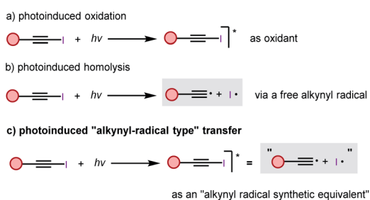
Scheme 1 Three possible reaction pathways.
