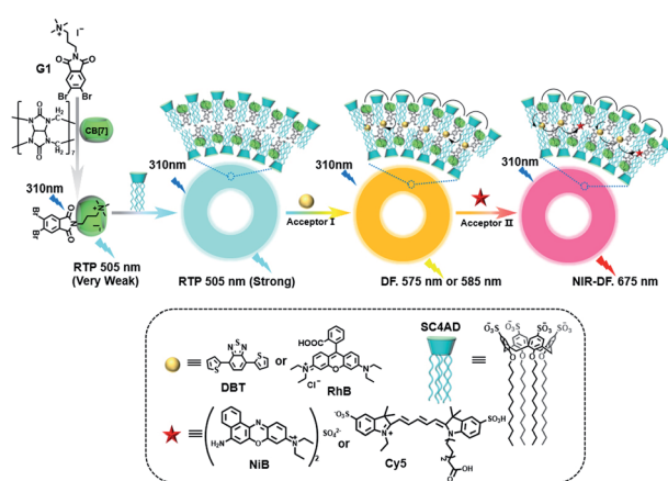
Fig. 16 Schematic illustration of construction of a two-stage light-harvesting phosphorescence energy transfer supramolecular assembly via SC4AH, CB[8], and di-bromophthalimide derivative.
