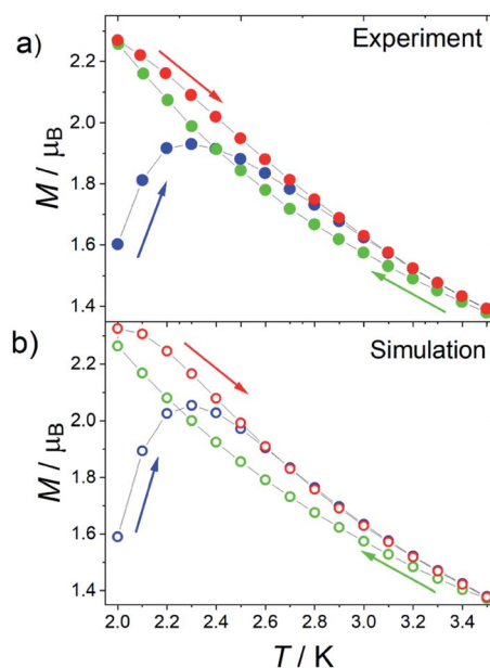
Fig. 6 (a) Experimental and (b) simulated ZFC (blue) and FC (green and red) curves of 1 at a sweeping rate of 0.03 K \text{s}^{-1} and at H = 1.6 \text{ kOe} . The arrows indicate the direction of the measurement for each curve.
