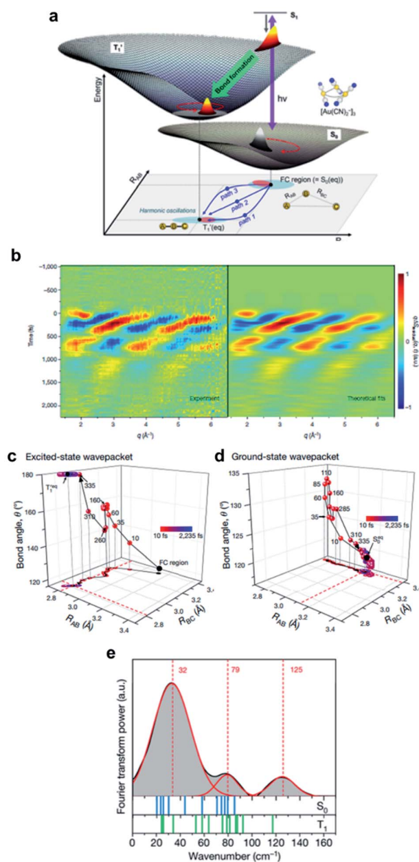
Fig. 19 (a) A schematic for the bond formation of [\text{Au}(\text{CN})_2]_3 upon photoexcitation. In the ground state, the trimer forms a loosely bound state. Upon photoexcitation, molecular vibration emerges along with the chemical bond formation. (b) Fs-TRXL data (left) for the molecular vibrations and the theoretical fits obtained using the ground-state ( S_0 ) and excited-state ( T_1 ) vibrations (right). (c and d) Wavepacket trajectories in real space for (c) the excited state and (d) the ground state. (e) Averaged experimental Fourier power spectrum (black) and the fits with three Gaussian functions (red). The blue and green lines indicate the vibrational frequencies of the ground and excited states obtained from the DFT calculation. Reproduced from ref. 63 with the permission of Springer Nature, copyright 2020.
