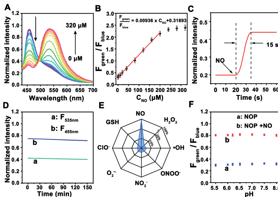
Fig. 2 (A) TPF emission spectra of the NOP with the addition of different concentrations of NO (0, 0.1, 10.0, 20.0, 40.0, 80.0, 120.0, 160.0, 200.0, 240.0, 280.0, and 320.0\text{ }\mu\text{M} ) in cell lysates. (B) Calibration curve between F_{\text{green}}/F_{\text{blue}} and various concentrations of NO ( n = 5 , S. D.). (C) Response time of the NOP with the addition of NO ( 50\text{ }\mu\text{M} ). (D) Photostability of the NOP at 455\text{ nm} ( F_{455\text{nm}} ) and 535\text{ nm} ( F_{535\text{nm}} ) after the NOP was exposed to a Xe lamp ( 90\text{ W} ). (E) Selectivity tests of the NOP toward common RNS ( 100\text{ }\mu\text{M} ) and ROS ( 100\text{ }\mu\text{M} ). (F) F_{\text{green}}/F_{\text{blue}} values of the NOP at pH 5.0\text{--}8.0 in the absence (a) and in the presence (b) of NO ( 50\text{ }\mu\text{M} ) ( n = 5 , S. D.).
