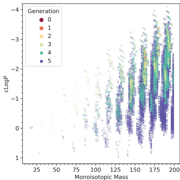
Fig. 5 Computed c\text{Log} P values as a function of molecular mass, colored by the generation in which the species are first produced. The network produces more and more hydrophobic species as it evolves.
