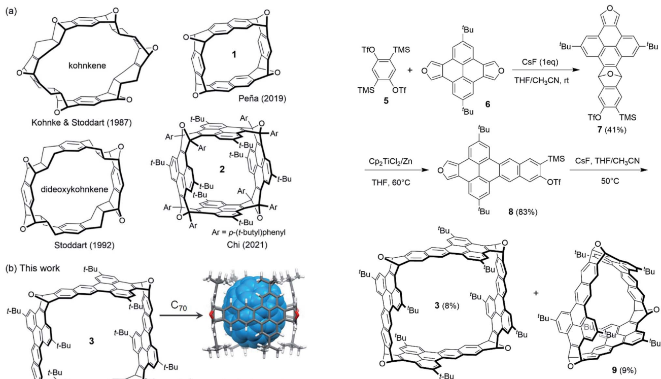
Scheme 1 Synthesis of 3.
