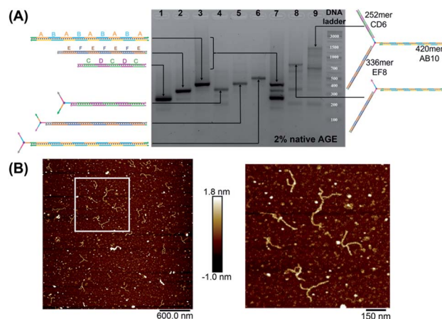
Fig. 2 Native agarose gel electrophoresis (AGE) characterization of mono-, bi- and tri-elongated "printed" junction ( T3 ) (A). Lanes 1, 2, 3: (CD) 3 (252 bps), (EF) 4 (336 bps) and (AB) 5 (420 bps) respectively; lanes 4, 5 and 6: T3 separately elongated by PCR with (CD) 3 (315 bps), (EF) 4 (399 bps) and (AB) 5 (483 bps), respectively. A-F are 42 base-pair building blocks of different sequences. Lanes 7 and 9: simultaneous PCR performed in the presence of (CD) 3 , (EF) 4 and (AB) 5 without T3 and with T3 (1071 bps), respectively. Lane 8: PCR product of (EF) 4 and (AB) 5 with T3 (819 bps). GeneRuler DNA ladder mix is used. (B) AFM characterization of "printed" junction with elongated arms in its double-stranded form. Note that the spherical structures are salts resulting from the surface drying, while the branched structures correspond to the extended junction.
