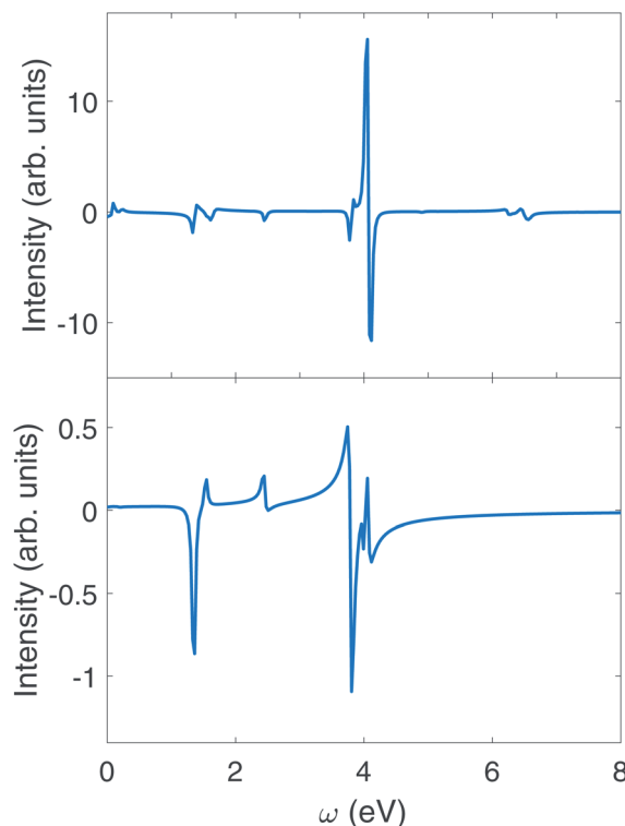
Fig. 8 CD signals eqn (9) of polariton in the chiral cavity with \delta = 0 , g = 1.028 \times 10^{-1} \text{ V } \text{\AA}^{-1} (or 0.002 \text{ a.u.} ) (top), and no cavity (bottom). The CD measurement follows a circularly polarized pump pulse in both polariton and bare molecule.
