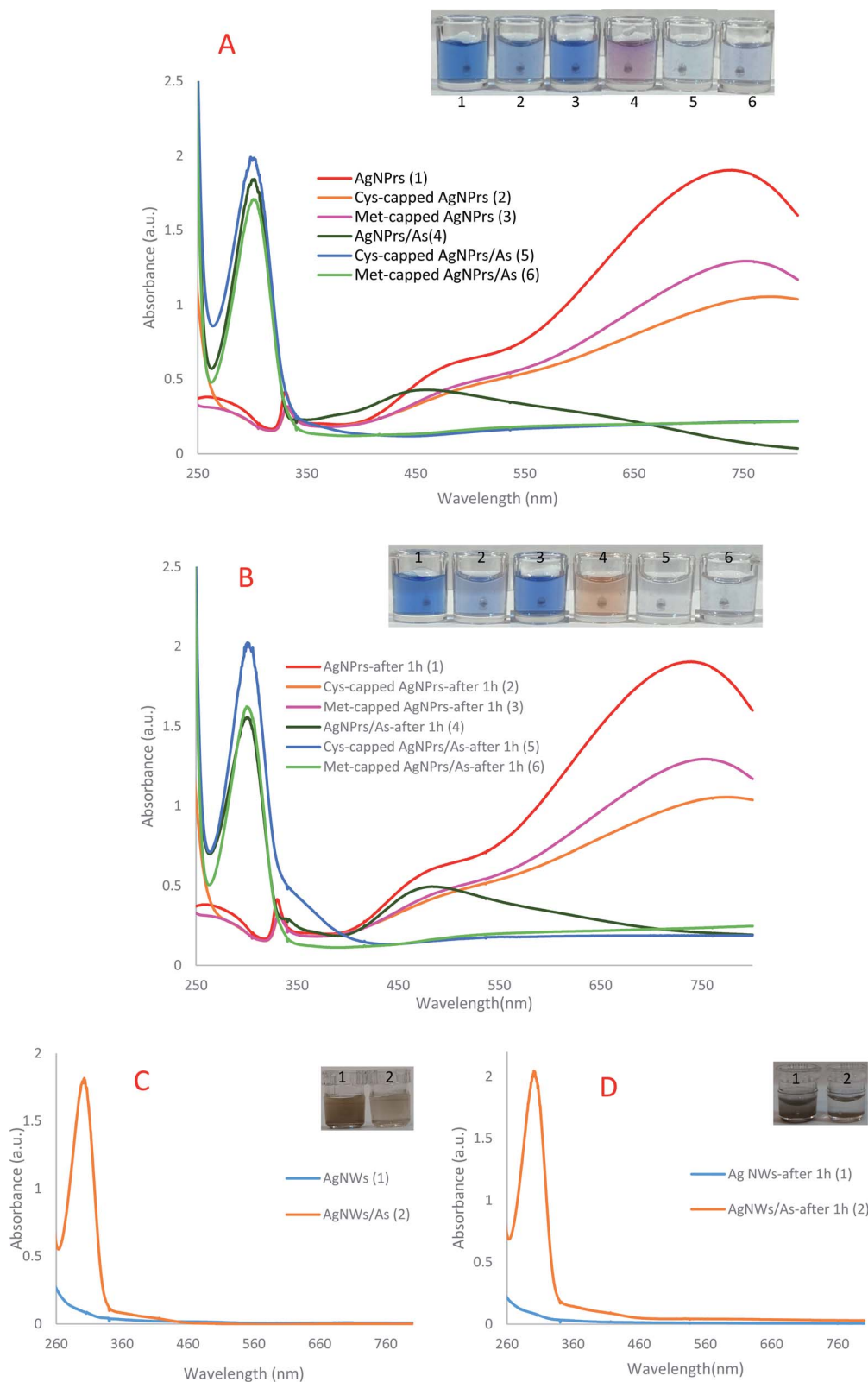
Fig. 1 The UV-Vis spectra of sensing probes in the presence and absence of arsenic (A) AgNPrs, Cys-capped AgNPrs, Met-capped AgNPrs; (B) AgNPrs, Cys-capped AgNPrs, Met-capped AgNPrs after 1 h; (C) AgNWs and (D) AgNWs after 1 h.
