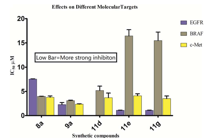
Fig. 1 Comparison of inhibitory activities ( IC_{50} \mu M ) of compounds on three targets.
