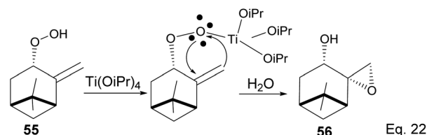
Scheme 18 Ti(OiPr)_4 -mediated intramolecular epoxidation of allylic peroxide.
