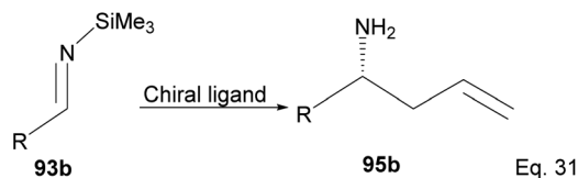
Scheme 27 \text{Ip}^2\text{B}(\text{allyl})\text{borane} promoted allylation of imine to amine.
