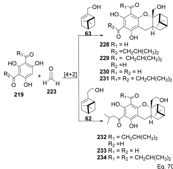
Scheme 64 Biomimetic synthesis of S -euglobals derivatives from nopol/myrtenol and o -quinone methide.
