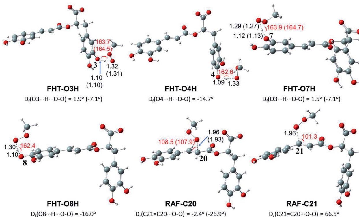
Fig. 4 Optimized structures of the transition states (TSs) for FHT and RAF reactions of rosmarinate mono-anion ( \text{RA}^- ) towards \text{CH}_3\text{OO}\cdot radicals in water calculated at the M05-2X/6-311++G(2df,2p) level of theory. D_f is the OHOO dihedral angle of the FHT TSs; D_r is the CCOO one of the RAF TSs. The values in parentheses correspond to the geometrical parameters obtained in the PEA phase.
