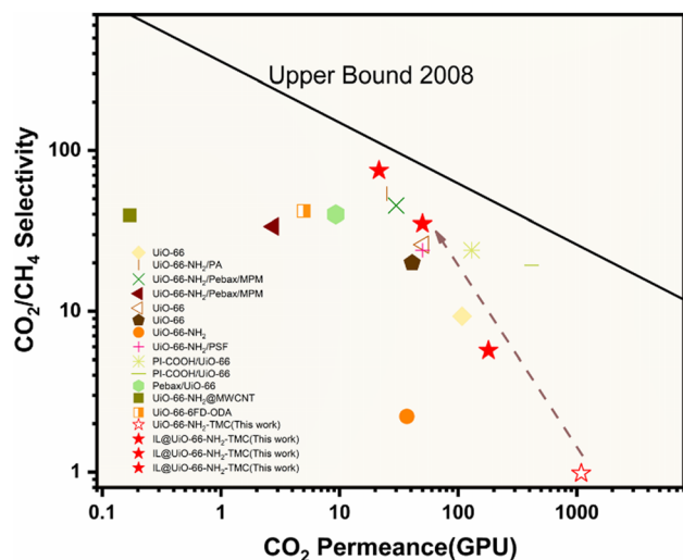
Fig. 10 Comparison of the \text{CO}_2/\text{CH}_4 separation performances between the IL@UiO-66-NH 2 -TMC membranes prepared in this study and other UiO-66 polycrystalline and composite membranes reported in the literature. Upper bound front drawn assuming a membrane thickness of 1 \mu\text{m} . Detailed information in this figure is listed in Table S3 (ESI†).
