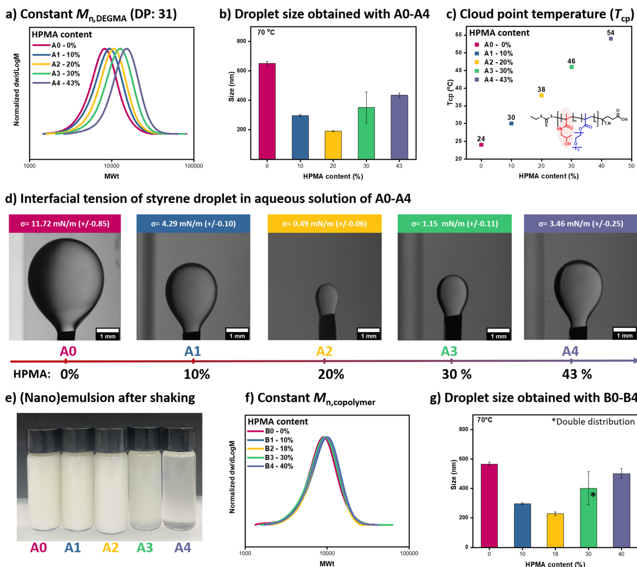
Fig. 2 (a) SEC traces of macro-CTAs A0–A4, (b) DLS sizes (by number at 70 °C) of (mini)emulsion formed by using A0–A4 with the following formulation: [macro-CTA] : [STY] : [SDS] = 25 mg : 35 \mu\text{L} : 0.25 mg, in 2 mL of deionized water (mass constant), (c) cloud point temperature of A0–A4, (d) interfacial tension of styrene droplet in an aqueous solution of macro-CTAs (A0–A4) measured by inverse pendant drop method, (e) pictures of (mini)emulsion formed by using A0–A4, (f) SEC traces of macro-CTAs B0–B4 and (g) DLS sizes (by number at 70 °C) of (mini)emulsion formed with B0–B4 with the following formulation: [macro-CTA] : [STY] : [SDS] = 1 (25 mg) : 97 (35 \mu\text{L} ) : 0.3 (0.25 mg), in 2 mL of deionized water.
