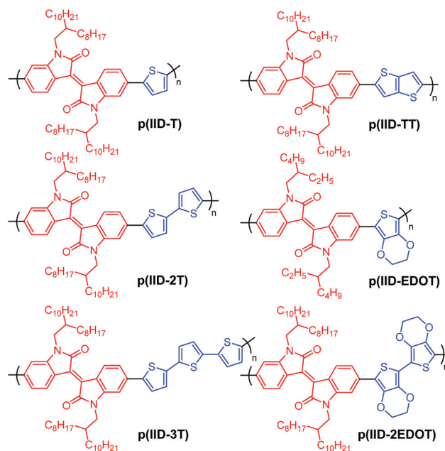
Scheme 1 Chemical structures of isosindigo-based polymers synthesized for the study of EC properties.
