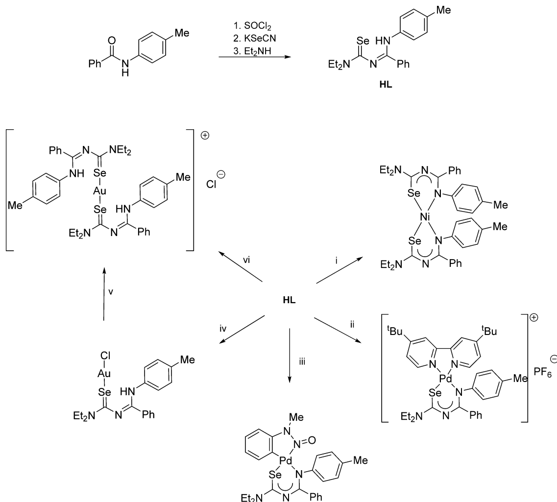
Scheme 5 (i) Ni(OAc) 2 . (ii) [PdCl 2 ( t Bu 2 bipy)], Et 3 N, NH 4 PF 6 . (iii) [Pd(OAc) 2 ](C 6 H 4 N(Me)N=O)] 2 . (iv) 0.5 eq. H[AuCl 4 ] or [AuCl(SMe 2 )]. (v) Standing in CDCl 3 . (vi) 0.5 eq. [AuCl(SMe 2 )].
