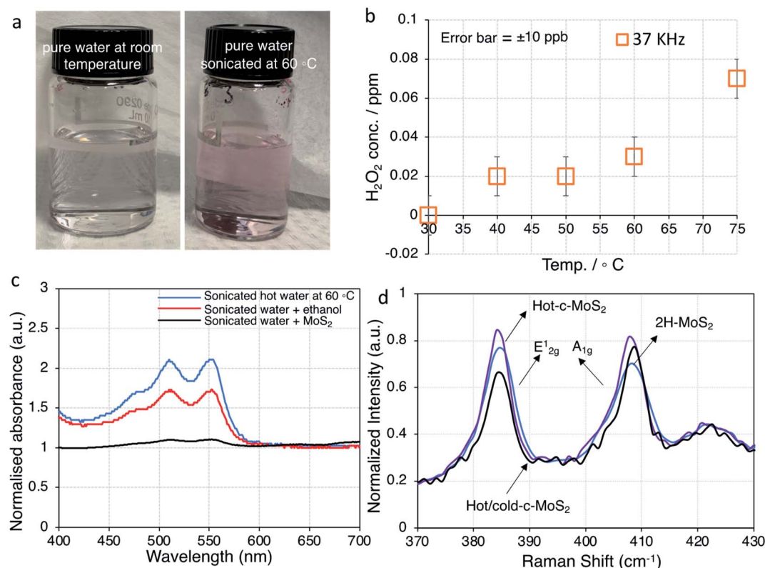
Fig. 3 Temperature dependent \text{H}_2\text{O}_2 formation in water and properties of \text{MoS}_2 . (a) photographic images of \text{H}_2\text{O}_2 formation in pure water at room temperature vs. sonicated hot water at 60^\circ\text{C} based on the colorimetric experiment; (b) amount of \text{H}_2\text{O}_2 formation as a function of temperature after sonication for 220 minutes. The error bars are given based on the display resolution of the instrument. (c) UV-visible spectra of samples sonicated at 37 kHz for 220 minutes; (d) Raman spectra of unsonicated, hot water sonicated, and hot & cold water sonicated 2\text{H}-\text{MoS}_2 samples. Spectra are normalized to the \sim 466\text{ cm}^{-1} peak.
