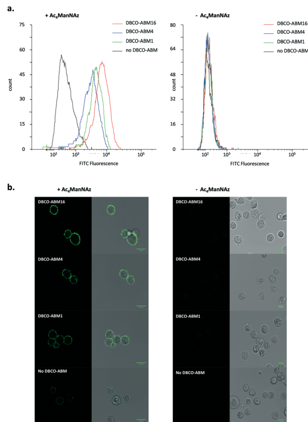
Fig. 2 a. Flow cytometry analysis of anti-Rha recruitment by labelled BT-549 cells with mono-, tetra- and hexadecavalent-ABMs. Azido cells were treated with 10 \mu M of DBCO-conjugates before incubation with HS. The antibody recruitment was revealed with AF488 conjugated secondary antibody. For both cases, non-labelled cells were used as control. b. Corresponding confocal microscopy images (scale bar: 10 \mu m ).
