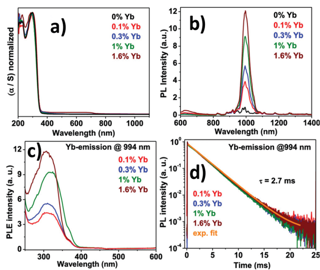
Fig. 8 (a) Absorption spectra, (b) PL spectra, (c) PLE spectra, and (d) PL decay dynamics of Yb doped \text{Cs}_2\text{AgInCl}_6 double perovskite MCs. Reproduced with permission. 77 Copyright 2019, American Chemical Society.
