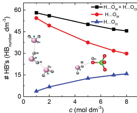
Fig. 4 Density of hydrogen bonds (HB's) as a function of the NaClO 4 molar concentration. The blue curve stands for H··OCl pairs (▲), the red curve for H··O w pairs (●), and the black curve (■) is the sum of both pairs.
