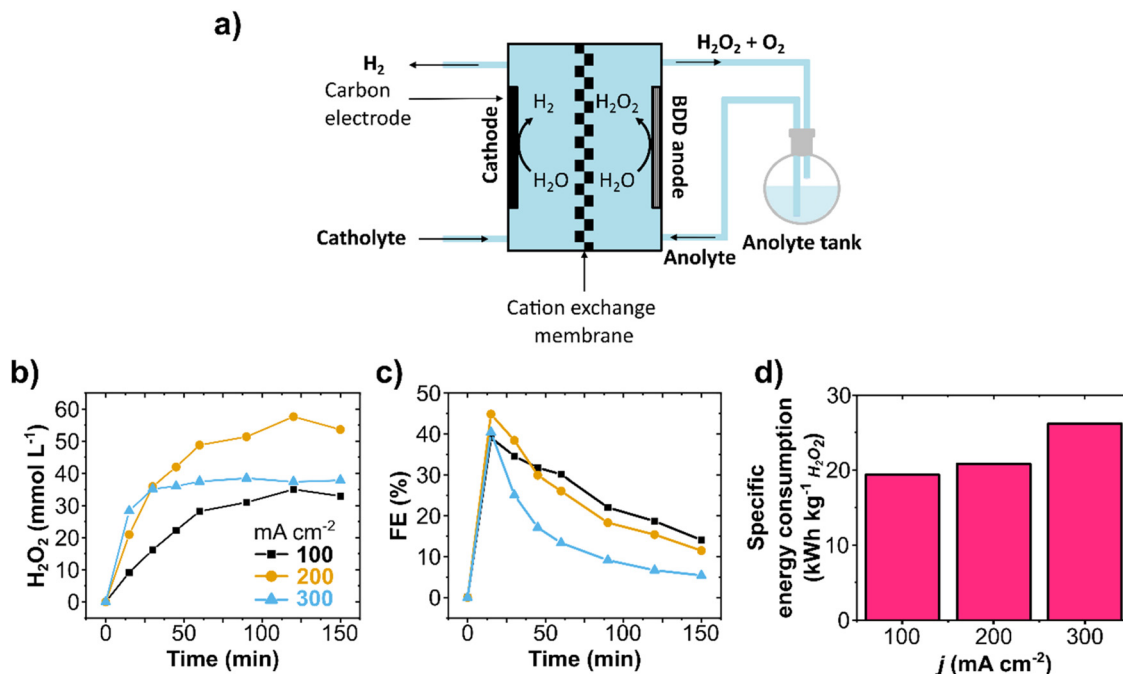
Fig. 2 Anodic H_2O_2 production in a circular flow reactor. (a) Schematic representation of the flow cell with circular flow. (b) H_2O_2 concentration and (c) FE obtained at different applied current densities. (d) Energy consumption to produce 1 kg of H_2O_2 based on the peak FE (at 15 min) at each applied current density. The flow cell was equipped with a carbon cathode and a BDD/Ta anode (both with a 10 cm 2 geometric area) separated by a Nafion 117 membrane. Each cell compartment contained a reservoir with 200 mL of 2 mol L -1 K_2CO_3 electrolyte circulating at 100 mL min -1 flow rate. 90 mmol L -1 Na_2SiO_3 was added to the anolyte as a chemical stabilizer to avoid H_2O_2 decomposition. The pH of the anolyte was kept constant at 12.6.
