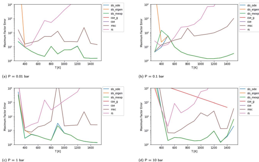
Fig. 4 Scores for each method at different pressures and temperatures for the acetyl + \text{O}_2 case study with the isomerization barrier lowered by 20 \text{ kcal mol}^{-1} . The CSE methods fail at most conditions in this case. The SLS methods overlap at high temperatures, with sls_eigen diverging at low temperatures.
