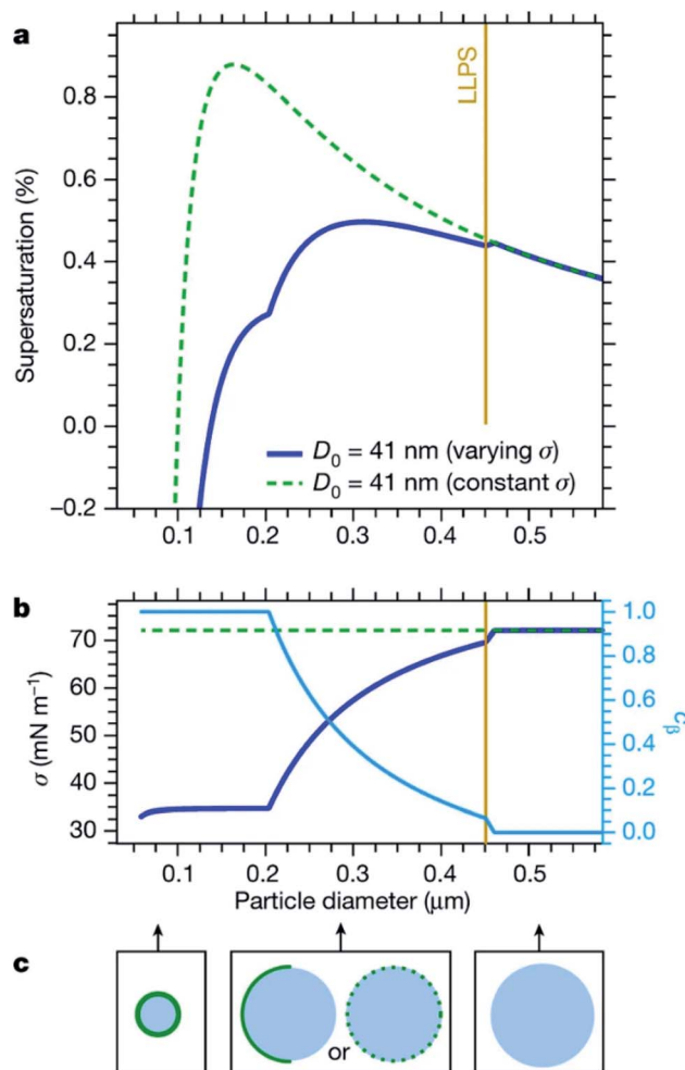
Fig. 7 Thermodynamic equilibrium modeling of an aerosol particle consisting of a 1 : 1 mass ratio of organic matter to sulfuric acid at 288.15 K and relative humidity of \text{RH} = 94\text{--}101\% . (a) Predicted Köhler curves of equilibrium supersaturation vs. particle diameter. The yellow vertical line marks the particle diameter at which liquid-liquid phase separation (LLPS) occurs. The dashed green curve shows the predicted Köhler curve for a droplet with a dry diameter of D_0 = 41 \text{ nm} and a constant surface tension equal to that of pure water ( \sigma = 72 \text{ mN m}^{-1} ). The solid blue curve shows predictions for a droplet with a dry diameter of D_0 = 41 \text{ nm} but a varying surface tension dependent on the size and phase of the particle. (b) The corresponding changes in surface tension as a function of particle diameter, with the predicted surface coverage of the organic layer ( c_p ) shown in light blue. (c) Cartoons of surface coverage as a function of particle diameter. Reprinted by permission from Springer Nature, Nature , Surface tension prevails over solute effect in organic-influenced cloud droplet activation, J. Ovadnevaite, A. Zuend, A. Laaksonen, K. J. Sanchez, G. Roberts, D. Ceburnis, S. Decesari, M. Rinaldi, N. Hodas, M. C. Facchini, J. H. Seinfeld and C. O' Dowd, Copyright 2017.
