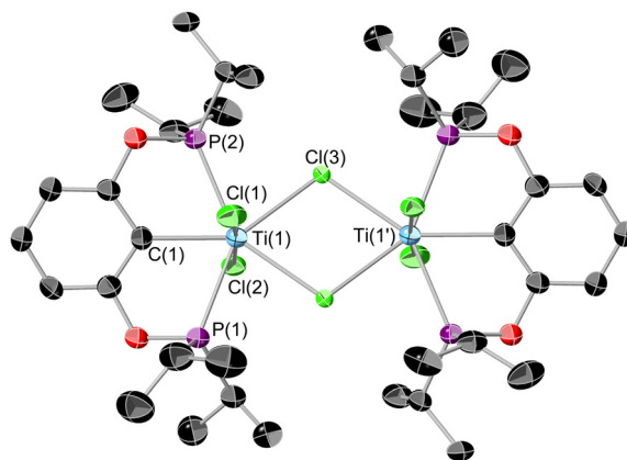
Fig. 5 ORTEP plot of 4. Thermal ellipsoids at 50% probability, hydrogens omitted for clarity. Selected bond lengths ( \text{\AA} ) and bond angles ( ^\circ ): Ti(1)–Cl(1) 2.293(1), Ti(1)–Cl(2) 2.336(1), Ti(1)–Cl(3) 2.587(1), Ti(1)–P(1) 2.578(1), Ti(1)–P(2) 2.587(1), Ti(1)–C(1) 2.252(4), Ti(1)–Ti(1') 4.116(1), \Sigma equatorial angles 360.89(5) , Cl(1)–Ti(1)–Cl(2) 174.05(5) .
