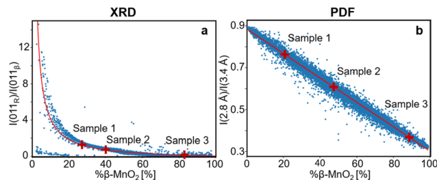
Fig. 5 (a) Intensity ratio between 011 R and 011 β lines from the modelled XRD patterns plotted against the β-MnO 2 fraction (%β-MnO 2 , blue dots) and fitted using eqn (3) (red solid line). (b) Intensity ratio between PDF peaks at 2.8 Å and 3.4 Å from the modelled PDFs plotted against %β-MnO 2 (blue dots) and fitted using a linear function (red solid line).
