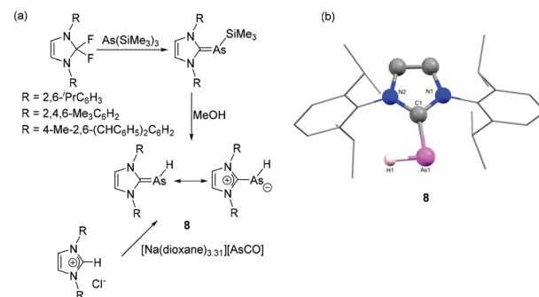
Fig. 4 (a) Synthesis of NHC-arsinidene 8 starting from [\text{AsCO}]^- and As( \text{TMS} ) 3 ; (b) solid-state structure of 8 .
