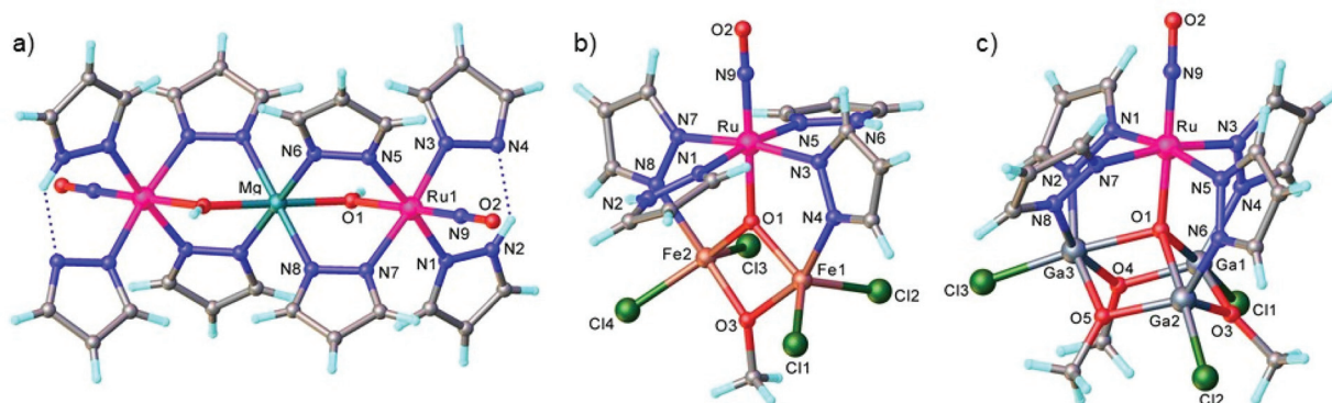
Fig. 10 The structures of (a) [\{\text{Ru}(\mu\text{-OH})(\mu\text{-pz})_2(\text{pz})(\text{NO})(\text{Hpz})\}_2\text{Mg}] , (b) [\text{Fe}_2\text{RuCl}_4(\mu_3\text{-O})(\mu\text{-O})(\mu\text{-pz})_2(\text{NO})(\text{Hpz})_2] and (c) [\text{Ga}_3\text{RuCl}_3(\mu_4\text{-O})(\mu\text{-OME})_3(\mu\text{-pz})_4(\text{NO})] . The structures are taken from those reported on the CSD; codes: (a) LAWGUP, (b) LAWHOK, (c) LAWHIE.
