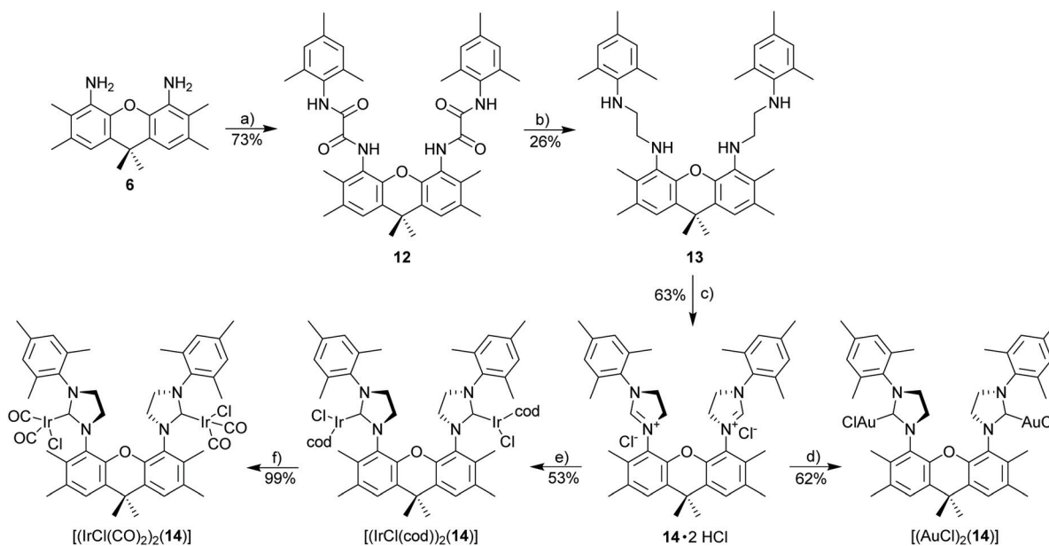
Scheme 5 Synthesis of imidazolium salt 14 ·2HCl and derived metal complexes. Reagents and conditions: (a) \text{MesNHC}(\text{O})\text{COCl} , \text{NEt}_3 , 0 °C to rt, 1 h; (b) \text{BH}_3 ·THF, reflux, 3 d; (c) triethyl orthoformate, \text{NH}_4\text{Cl} , 110 °C, 24 h; (d) [\text{AuCl}(\text{SMe}_2)] , \text{K}_2\text{CO}_3 , acetone/ \text{CH}_2\text{Cl}_2 , 50 °C; (e) [\text{IrCl}(\text{cod})_2] , \text{K}_2\text{CO}_3 , acetone/ \text{CH}_2\text{Cl}_2 , 50 °C; (f) CO, 0 °C, 30 min, \text{CH}_2\text{Cl}_2 .
