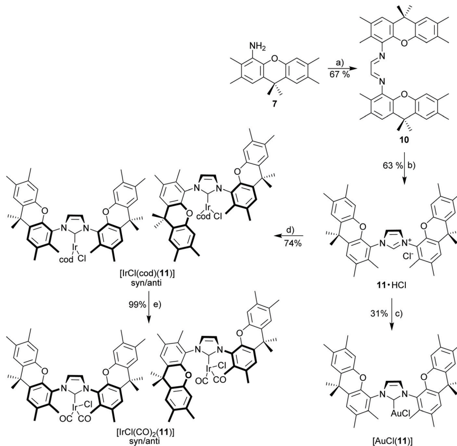
Scheme 4 Synthesis of imidazolium salt 11 ·HCl and derived metal complexes. Reagents and conditions: (a) glyoxal, p TsOH, EtOH, 50 °C; (b) paraformaldehyde, \text{Me}_3\text{SiCl} , EtOAc, 70 °C, 24 h; (c) [\text{AuCl}(\text{SMe}_2)] , \text{K}_2\text{CO}_3 , acetone, 50 °C; (d) [\text{IrCl}(\text{cod})_2] , \text{K}_2\text{CO}_3 , acetone, 50 °C; (e) CO, 0 °C, 30 min, \text{CH}_2\text{Cl}_2 .
