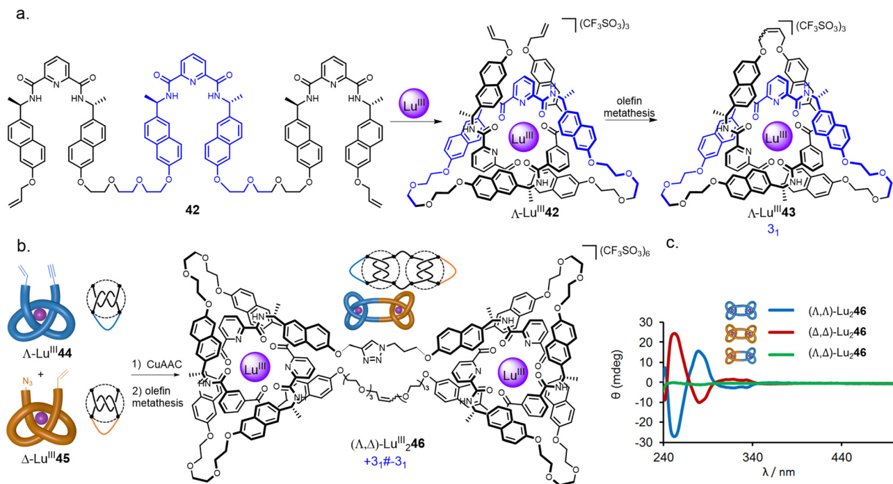
Fig. 15 (a) Synthesis of trefoil knot \Lambda - \text{Lu}^{\text{III}} 43 by folding a single ligand around a lanthanide ion. 80 (b) Stereoselective synthesis of composite knots with tangle representations, here represented by square knot synthesis. 82 (c) CD spectra of granny and square knots \text{Lu}_2 46. 82 Reproduced from ref. 82 through a CC-BY license.
