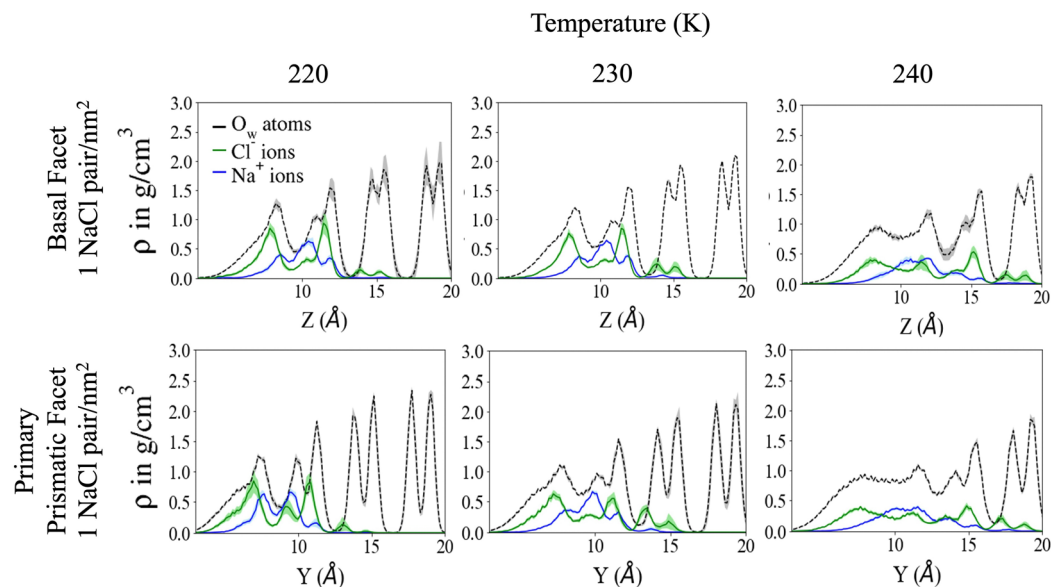
Fig. 3 \text{Cl}^- and \text{Na}^+ density profiles for the three highest temperatures sampled for both the basal and primary prismatic facet at the \text{NaCl} surface density of 1 \text{ NaCl pair nm}^{-2} . Respective oxygen atom density profiles are included to show where the density of the ions is in relation to the bilayers. Ion density is scaled by a factor of 5\times . The shaded regions corresponds to the standard deviation of the density profiles from block statistical analysis.
