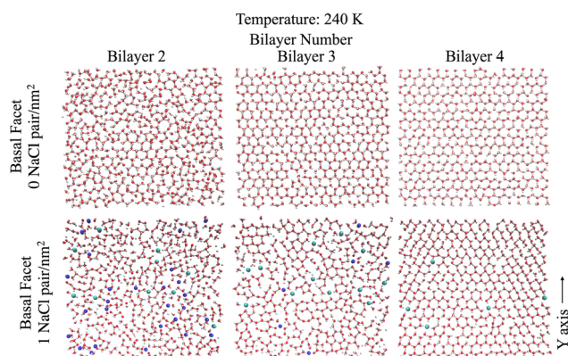
Fig. 4 Snapshots from a top down view of the second, third, and fourth bilayers of the basal facet with and without \text{NaCl} at 240 K. Bonds shown are for a bond length cutoff 1.9 \text{ \AA} to display the crystalline structure (or lack thereof) in each layer. \text{Na}^+ ions are represented by blue spheres and \text{Cl}^- ions are represented by green spheres.
