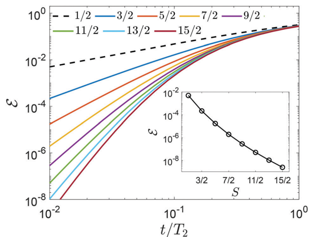
Fig. 1 Error \epsilon after QEC as a function of the memory time t (in units of T_2 ), for different values of S . In this simulation, the system is prepared in the state |\psi_0\rangle = (|0_L\rangle + |1_L\rangle)/\sqrt{2} and evolves subject to pure dephasing for a time t . The capacity of the code increases with S , as shown in the inset for fixed t/T_2 = 10^{-2} .
