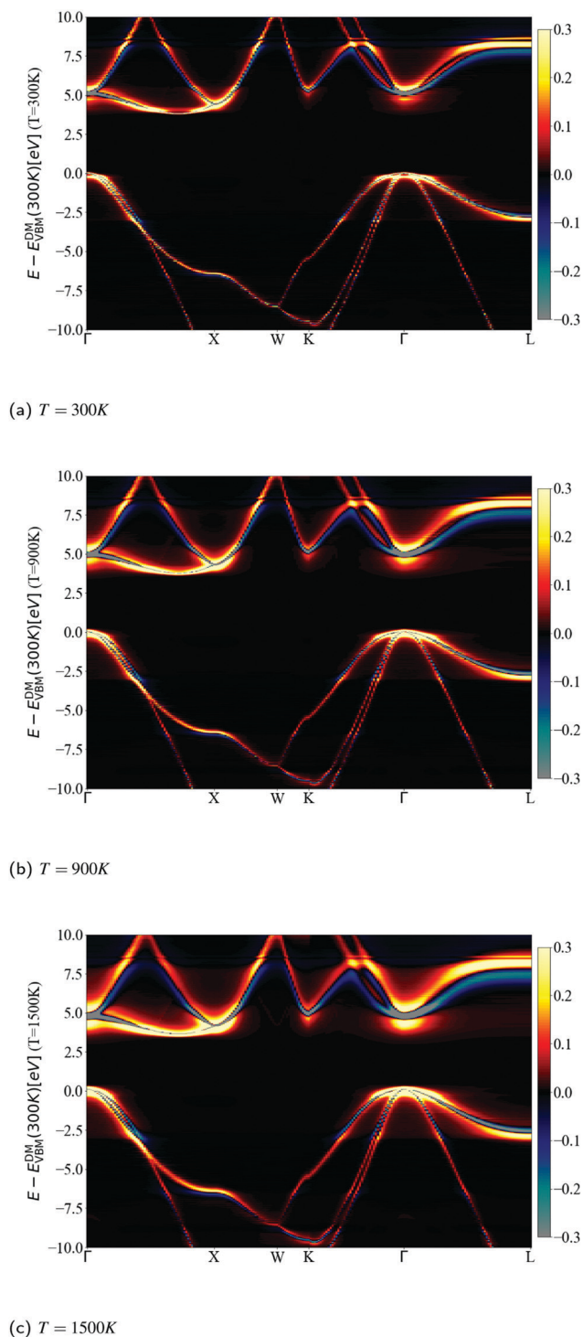
Fig. 13 Calculated spectral function difference between the CE and DM, A^{CE}(\omega) - A^{DM}(\omega) at (a) 300 K, (b) 900 K, and (c) 1500 K. To highlight the nonpolaronic signature near the VBM and CBM, the intensity scale of the density of states (colormap) was limited to \pm 0.3 . For positive values (red and yellow colors), the CE has more intensity than DM, and the opposite happens for the negative values (blue and grey colors). Comparatively with the narrow bands of DM, the CE approach has a much broader spread of the QP weight. Around most of the high symmetry k -points the broadening is almost symmetric, except L , where it is asymmetric, creating a tail.
