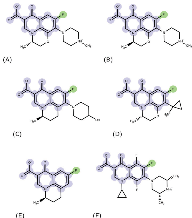
Fig. 1 Examples of FQ structures: (A) levofloxacin (LFX), (B) ofloxacin (OFX), (C) nadifloxacin (NFX), (D) pazufloxacin (PFX), (E) flumequinone (FMQ), and (F) orbifloxacin. The molecular scaffold common to all quinolones and the fluorine atom characterizing fluoroquinolones are highlighted in blue and green, respectively.
