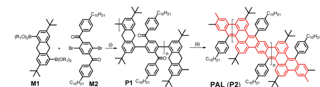
Scheme 2 Synthesis of a conjugated hydrocarbon ladder polymer PAL (P2) with a polyacene skeleton; the boronic esters are preferably pinacolates ( R_1 – R_2 : CMe_2 – CMe_2 ); (i) Pd(PPh_3)_4 , K_2CO_3 , toluene/ H_2O , (ii) KOC(CH_3)_3 /DMF.
