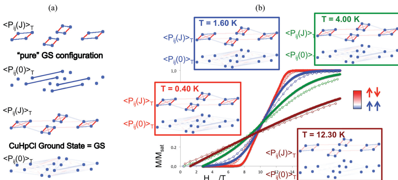
Fig. 7 (a) Short-range \langle P_{ij}(J) \rangle_T and long-range \langle P_{ij}(0) \rangle_T spin correlations between magnetic units for pure singlet ground state GS configuration and \text{CuHpCl} ground state GS configuration. (b) Temperature dependence of the magnetic correlation between all spin units at 0.40, 1.60, 4.00, and 12.30 K (in accordance to the magnetization experimental data). Notice that spins coupled are represented in red, and spins arranged parallel in blue.
