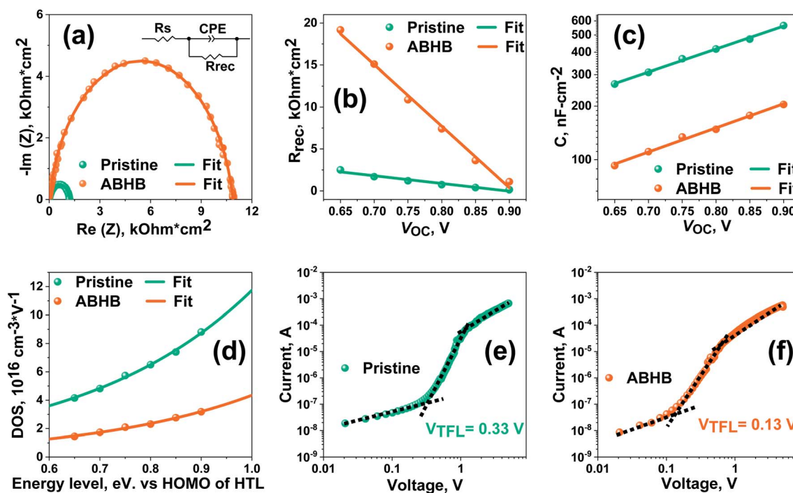
Fig. 6 (a) Nyquist plots of the devices with and without ABHB. (b) R_{\text{rec}} variation with different biases, (c) variation of C with variable bias, and (d) trap density of states (DOS) versus electron energy level. (e and f) dark J – V characteristics from hole-only devices of pristine and ABHB modified devices respectively.
