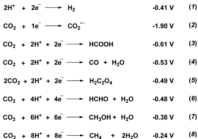
Scheme 2 Electrochemical reaction equations (all potentials vs. NHE at pH 7).
