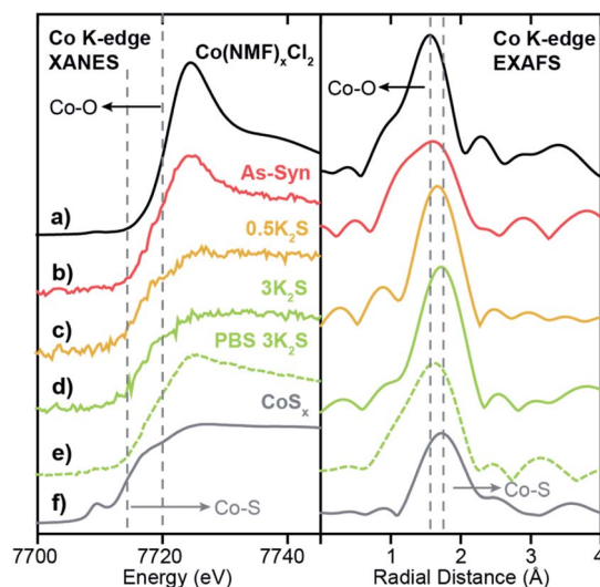
Fig. 4 Co K-edge XANES and EXAFS spectra for (a) Co(NMF)_xCl_2 , (b) As-synthesized 0.3Co- WS_2 , (c) 0.3Co- WS_2 annealed with 0.5 equiv. of K_2S , (d) 0.3Co- WS_2 annealed with 3.0 equiv. of K_2S , (e) 0.3Co- WS_2 3 K_2S immersed in 1 M PBS electrolyte, and (f) amorphous CoS_x . Dotted lines indicate the edge energies or scattering peaks for Co-O and Co-S coordination.
