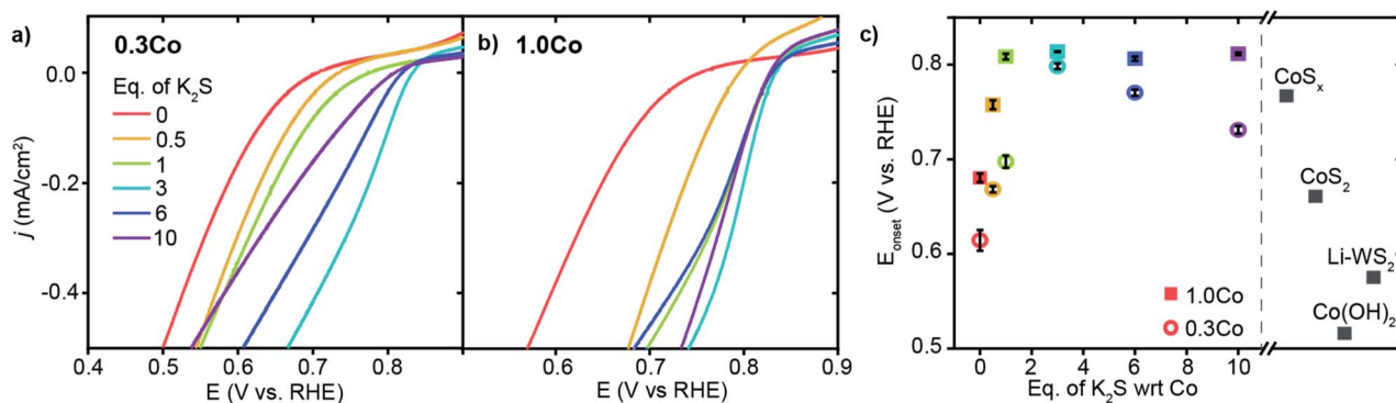
Fig. 3 Oxygen reduction reaction activity in O_2 -saturated 1 M PBS (pH = 7) electrolyte. (a and b) ORR LSVs for the full series of 0.3Co and 1.0Co- WS_2 samples treated with K_2S , (c) E_{onset} vs. equivalents of K_2S for Co- WS_2 catalysts compared to Co and WS_2 control samples.
