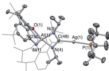
Fig. 4 Molecular structure of 5-Ag in the solid state as determined by X-ray crystallography. Thermal ellipsoids set at the 50% probability level. Hydrogen atoms omitted and {}^1\text{Pr}/{}^t\text{Bu} shown in wireframe for clarity. Key bond lengths (Å) and angles (°): Ag(1)–C(48): 2.118(2), Ag(1)–P(1): 2.3851(6), N(3)–C(48): 1.346(3), N(4)–C(48): 1.345(3).
