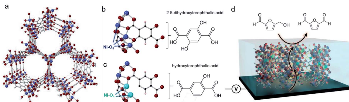
Fig. 1 Ni-MOF 74 contains cylinder shaped pores and chains of 5-coordinate Ni oxide units (a). The 2,5-dihydroxyterephthalic acid organic linker, will bind through both the carboxylate and alcohol units (b) and replacing it with 2-hydroxyterephthalic acid will result in defect sites of 4-coordinate Ni sites (c). We studied the effects of these defect sites with electrochemical and spectroscopic techniques, using the oxidation of HMF as a model reaction (d).
