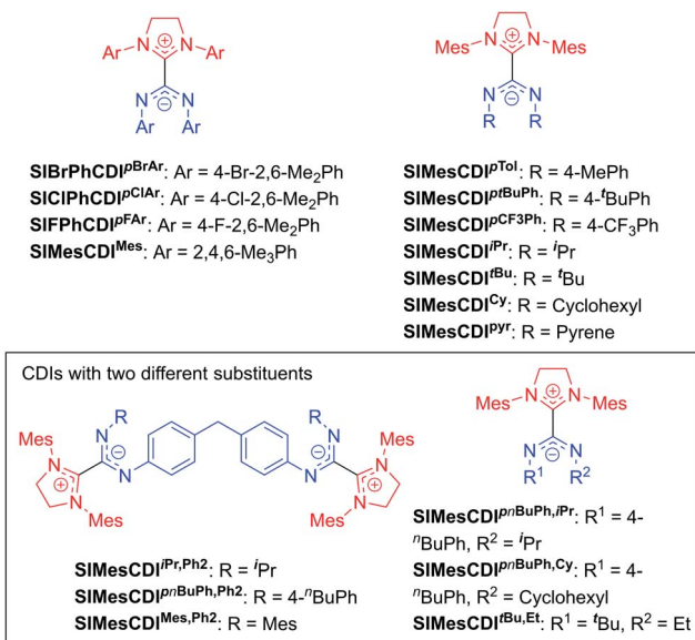
Fig. 5 Previously synthesized imidazolidin-2-ylidene based discrete NHC-CDI adducts.
