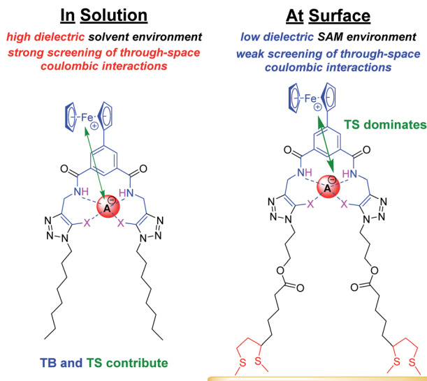
Fig. 6 Schematic representation of through-bond (TB, blue) and through-space (TS, green arrows) interactions that drive anion recognition in the cationic state of 1.XB / HB in solution and at 2.XB / HB SAM . In the more polar solvent environment of high dielectric the TS contribution is diminished and TB contributions are significant. In the low dielectric SAM environment, TS contributions are strongly enhanced such that binding in the cationic state is switched-on more strongly, inducing a larger sensor response.
