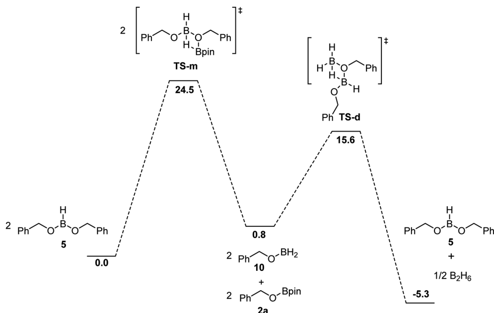
Fig. 5 Free energies in kcal \text{mol}^{-1} for the proposed mechanism of the formation of 2a and regeneration of \text{BH}_3 calculated at DFT/ \omega\text{B97XD}/6\text{-}31+\text{G}^{**} (SMD, tetrahydrofuran) level of theory.
