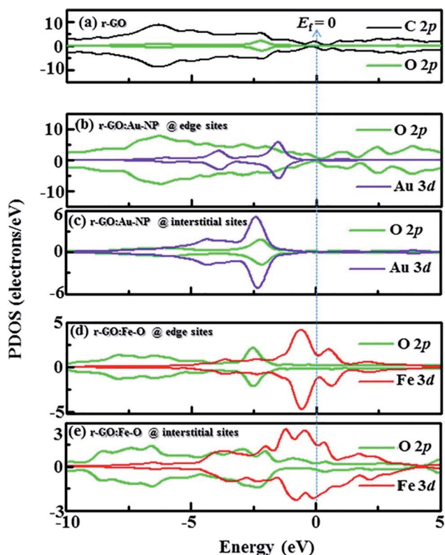
Fig. 29 Partial density of states (PDOS) showing contribution from C, Au, Fe, and O orbitals in (a) r-GO, (b) r-GO: Au at edge sites, (c) r-GO: Au at interstitial sites, (d) r-GO: Fe–O at edge sites and (e) r-GO: Fe–O at interstitial sites [minimal contributing orbitals to the PDOS are C 2s, O 2s, Au 4s and Fe 2p (not shown)]. This figure is reproduced from ref. 193 with permission from Elsevier, copyright 2020.
